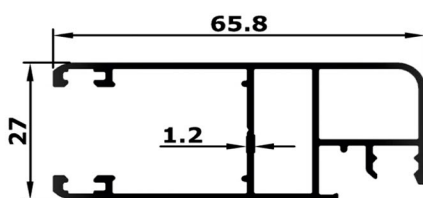
ZALI HANDLE
