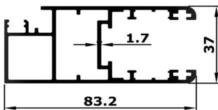
ZALI HANDLE
