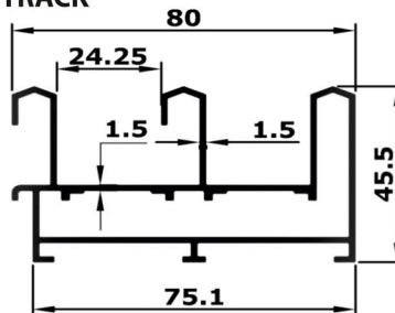
3 TRACK
