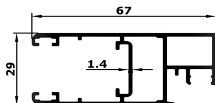
ZALI HANDLE
