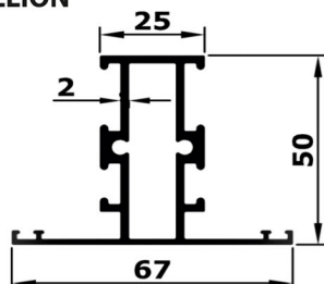
MULLION
