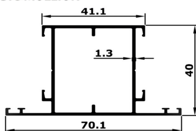
BIG MULLION
