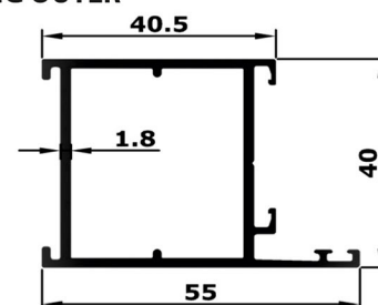
BIG OUTER
