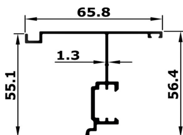
FLYING MULLION
