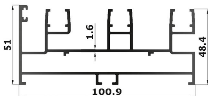
3 TRACK
