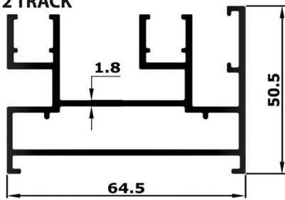
2 TRACK
