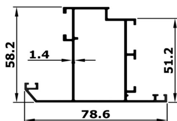
WINDOW MULLION
