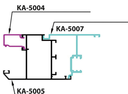
ASSEMBLY
