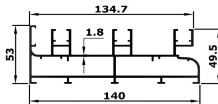
3 TRACK
