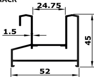
2 TRACK
