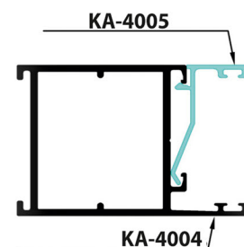
ASSEMBLY
