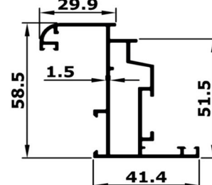
WINDOW Z
