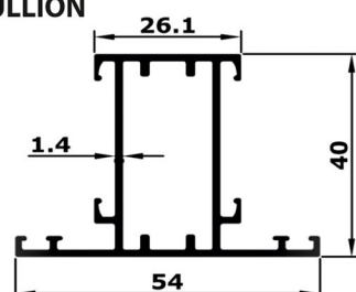
MULLION
