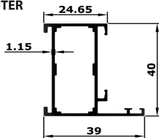
OUTER
