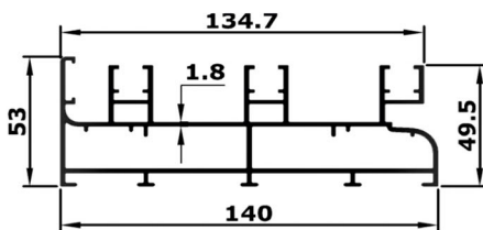
3 TRACK
