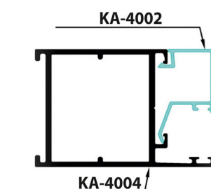
ASSEMBLY
