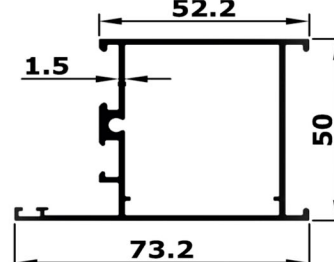
BIG OUTER
